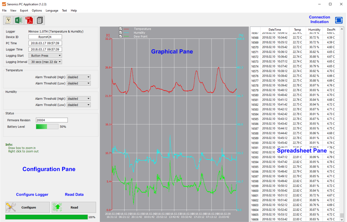
Figure 4: Senonics GUI
