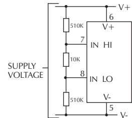
Check Link 2 is OPEN . Measuring a supply voltage. (min. 7.5V, max. 14V).
