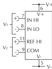
Check Links 1 & 4 are OPEN . Measuring the ratio of two voltages. Reading = 1000 V_1/V_2 50mV < V_2 < 200mV V_1 < 2V_2 .
