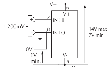
Check Link 2 is OPEN . Split supply operation.
