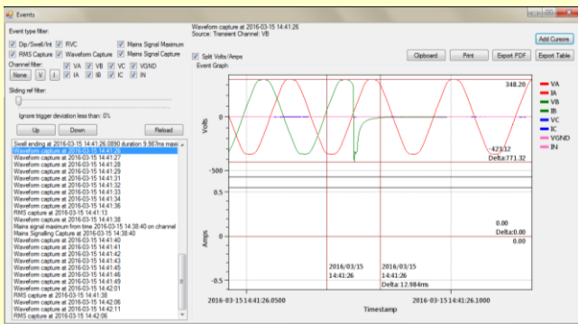
Figure 2: CITRUS - Event - waveform capture
