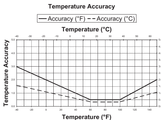
Figure 2. Temperature Accuracy
